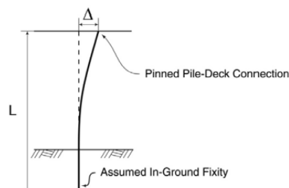
FIGURE 31F-7-15—ASSUMED IN-GROUND FIXITY
