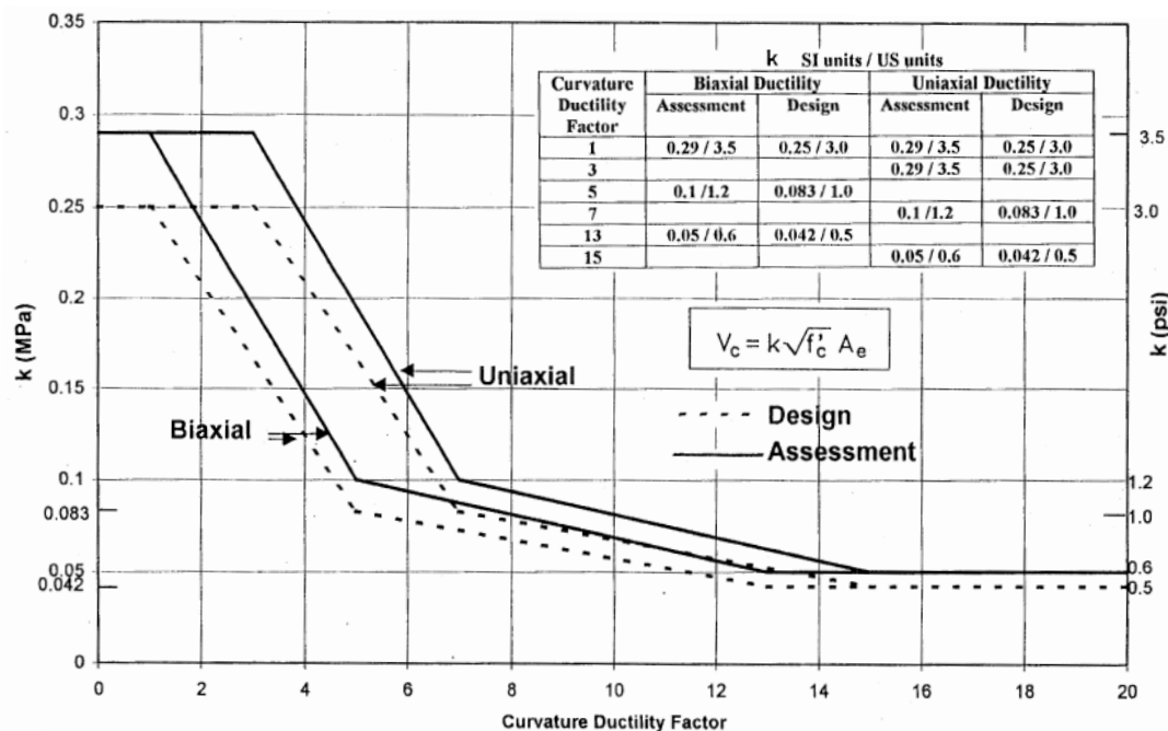
FIGURE 31F-7-6—CONCRETE SHEAR MECHANISM (from Fig. 3-30 of [7.2])
