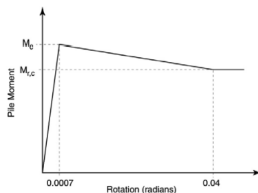
FIGURE 31F-7-12—JOINT ROTATION
