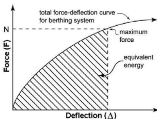
FIGURE 31F-5-5—BERTHING ENERGY CAPACITY
