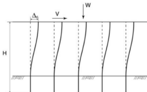
FIGURE 31F-4-8—P-Δ EFFECT
