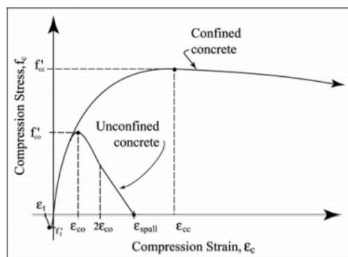
FIGURE 31F-7-1—STRESS-STRAIN CURVES FOR CONFINED AND UNCONFINED CONCRETE [7.1]
