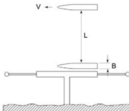
FIGURE 31F-5-4—PASSING VESSEL
