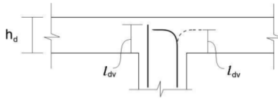
FIGURE 31F-7-9—DEVELOPMENT LENGTH
