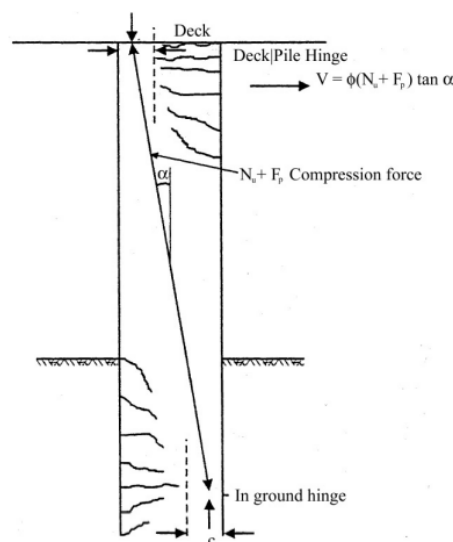
FIGURE 31F-7-8—AXIAL FORCE SHEAR MECHANISM
