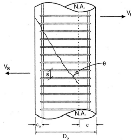
FIGURE 31F-7-7—TRANSVERSE SHEAR MECHANISM
