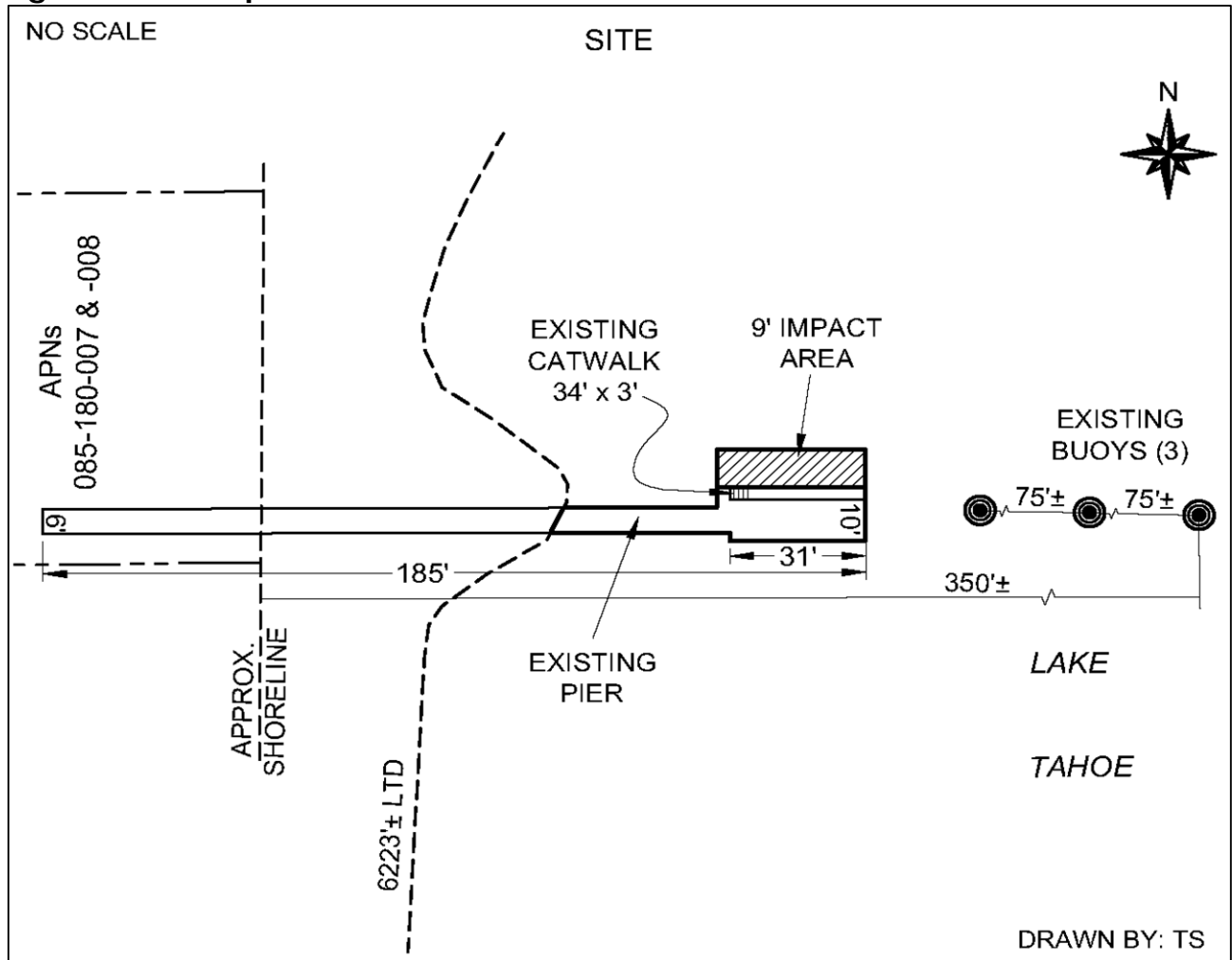
Figure 2. Site Map
