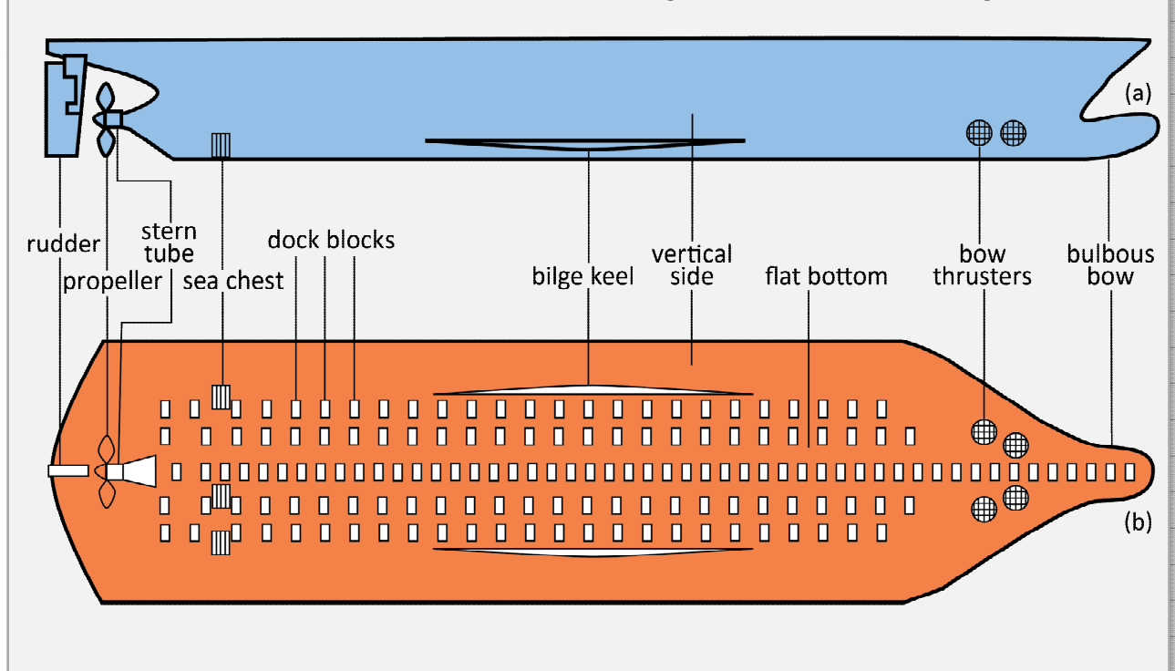
Figure 6-1. Niche areas susceptible to biofouling accumulation. a) Side view of a vessel. b) Bottom view of a vessel. Figure originally from Davidson et al. 2016.
