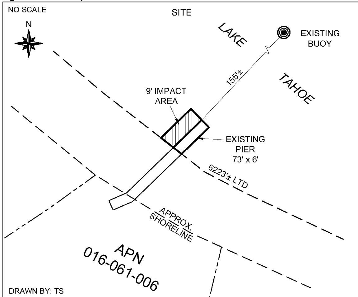
Figure 2. Site Map
