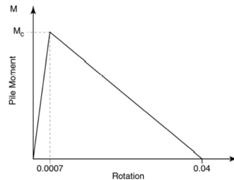
FIGURE 31F-7-11 REDUCED PILE MOMENT CAPACITY
