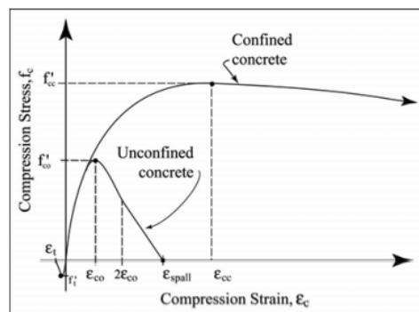
FIGURE 31F-7-1 STRESS-STRAIN CURVES FOR CONFINED
