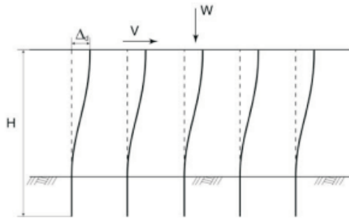
FIGURE 31F-4-8 P-Δ EFFECT
