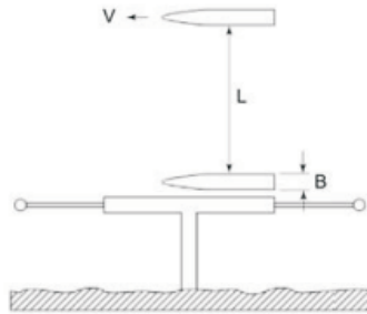
FIGURE 31F-5-4 PASSING VESSEL
