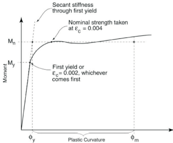
FIGURE 31F-7-5 MOMENT CURVATURE ANALYSIS
