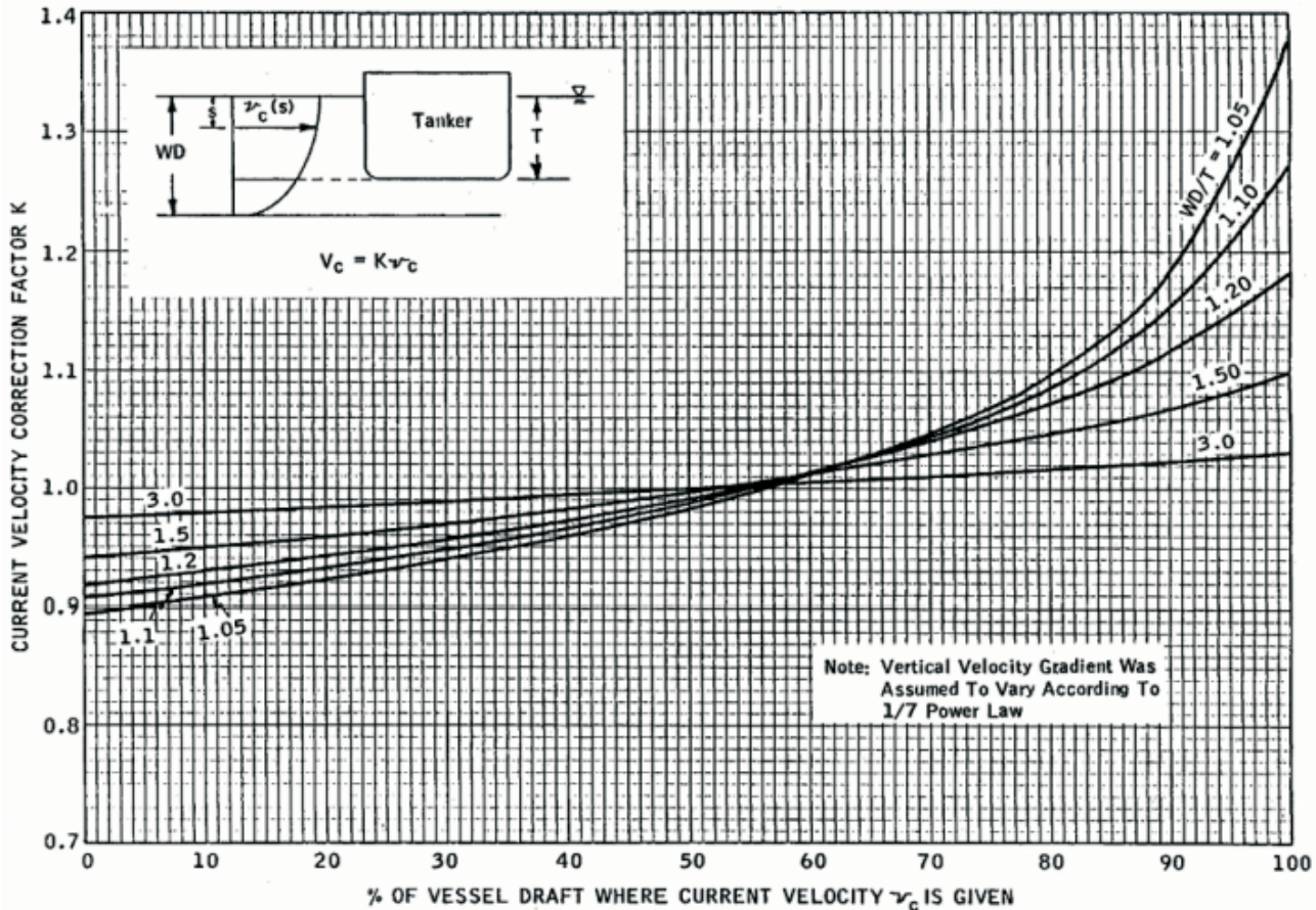
FIGURE 31F-3-4 CURRENT VELOCITY CORRECTION FACTOR (p. 23, OCIMF, 1997 [3.13])
