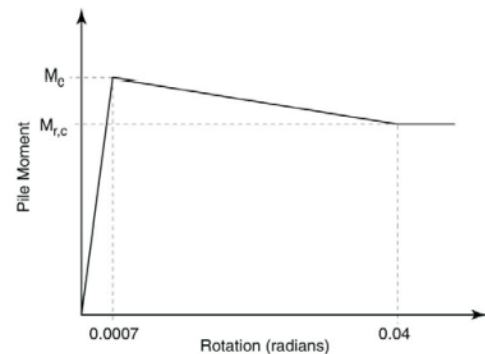
FIGURE 31F-7-12 JOINT ROTATION
