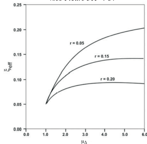
FIGURE 31F-4-3 RELATION BETWEEN DUCTILITY, \mu_\Delta , AND EFFECTIVE DAMPING, \xi_{\text{eff}} [4.1]
