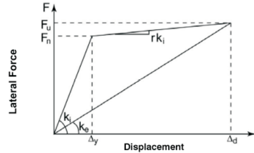
FIGURE 31F-4-5 EFFECTIVE STIFFNESS, k_e [4.1]
