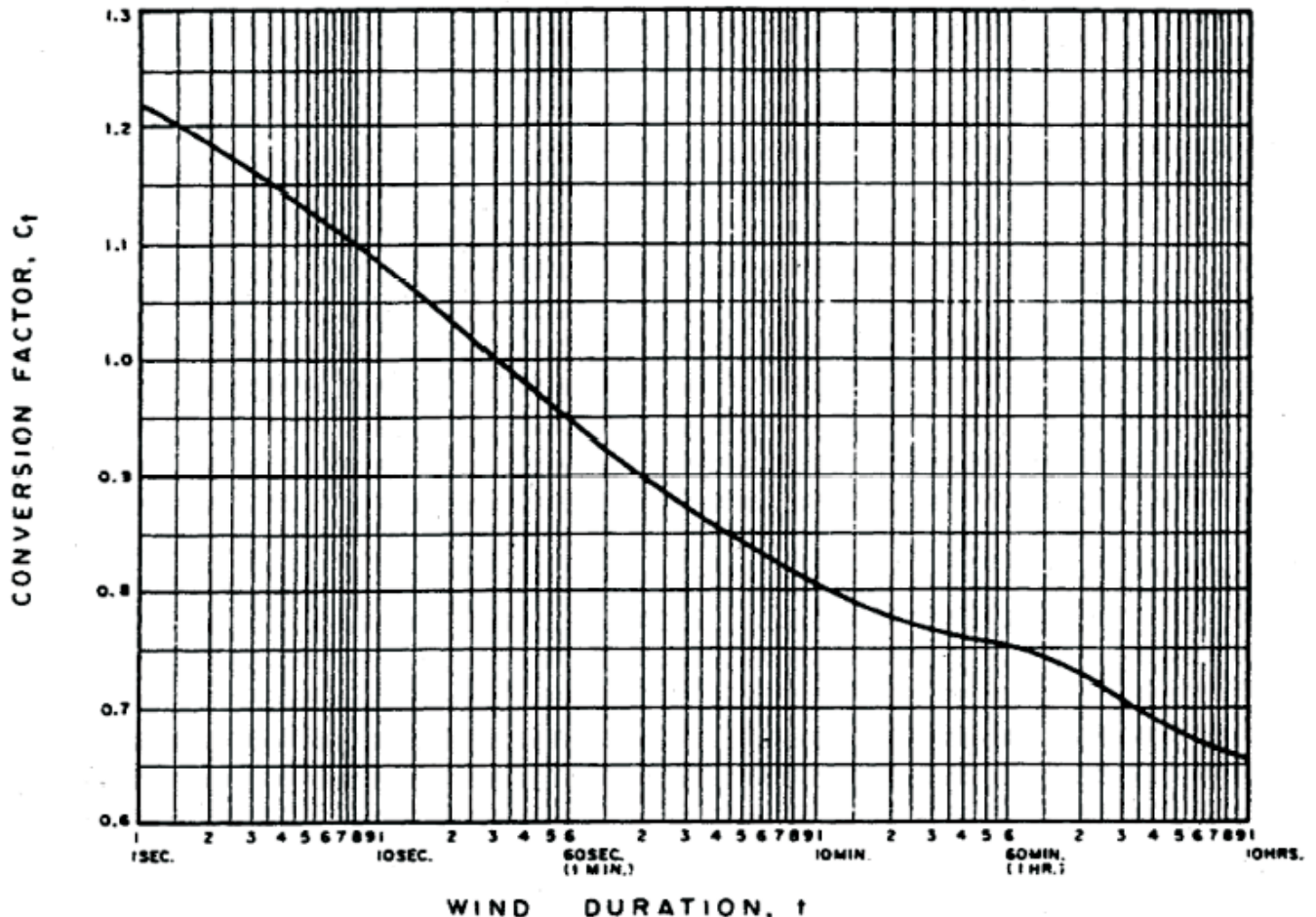
FIGURE 31F-3-3 WIND SPEED CONVERSION FACTOR [3.12]
