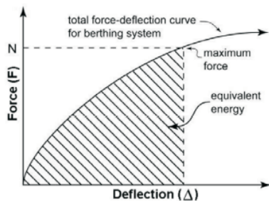
FIGURE 31F-5-5 BERTHING ENERGY CAPACITY
