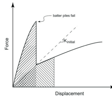
FIGURE 31F-7-14 PUSHOVER CURVE FOR ORDINARY BATTER PILES
