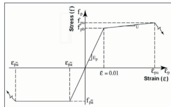
FIGURE 31F-7-3 STRESS-STRAIN CURVE FOR PRESTRESSED STEEL [7.4]
