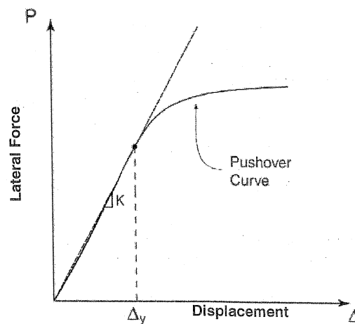
FIGURE 31F-4-6—STIFFNESS FOR LINEAR MODAL ANALYSIS
