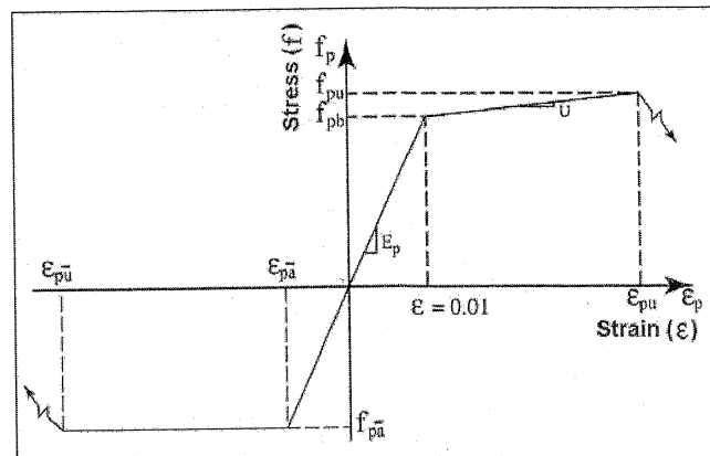
FIGURE 31F-7-3—STRESS-STRAIN CURVE FOR PRESTRESSED STEEL [7.4]
