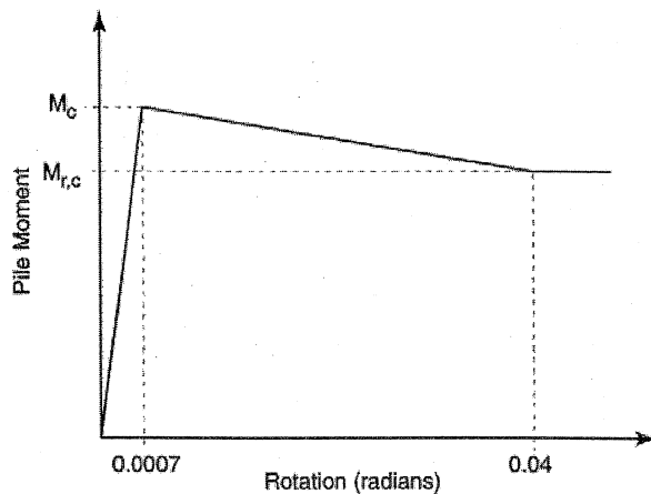
FIGURE 31F-7-12—JOINT ROTATION
