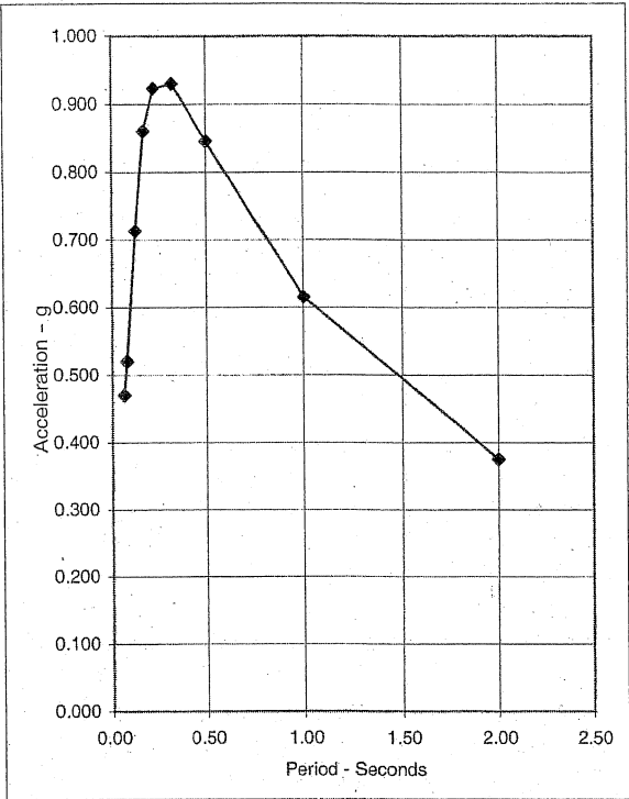
FIGURE 31F-3-1—RESPONSE SPECTRA FOR THE PORTS OF LOS ANGELES AND LONG BEACH, 475 YEAR RETURN PERIOD (5% Critical Damping)
