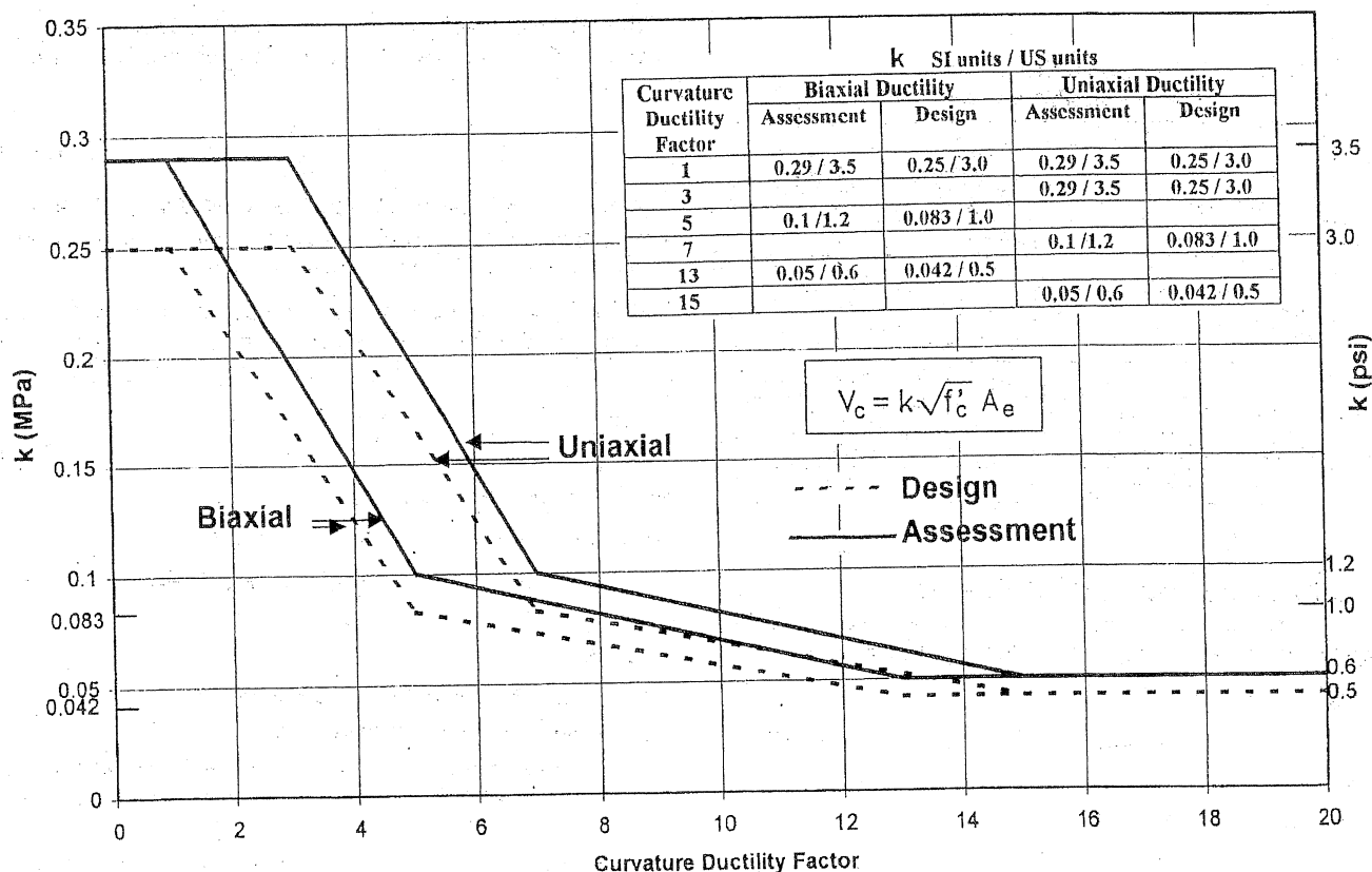
FIGURE 31F-7-6—CONCRETE SHEAR MECHANISM (from Fig. 3-30 of [7.2])
