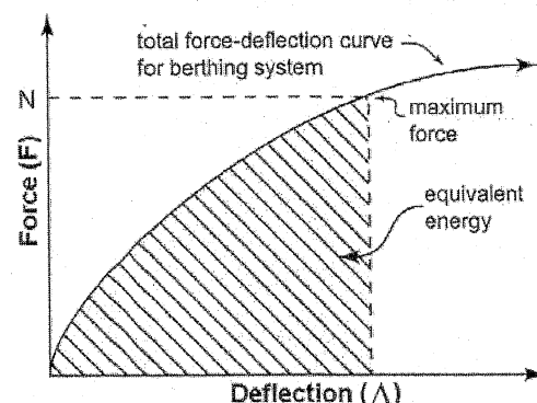
FIGURE 31F-5-5—BERTHING ENERGY CAPACITY
