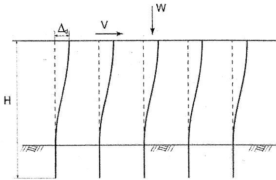
FIGURE 31F-4-8—P-Δ EFFECT
