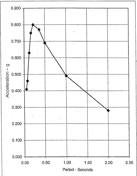
FIGURE 31F-3-2—RESPONSE SPECTRA FOR PORT HUENE, 475 YEAR RETURN PERIOD (5% Critical Damping)
