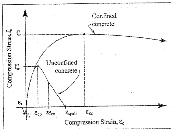
FIGURE 31F-7-1—STRESS-STRAIN CURVES FOR CONFINED AND UNCONFINED CONCRETE [7.1]
