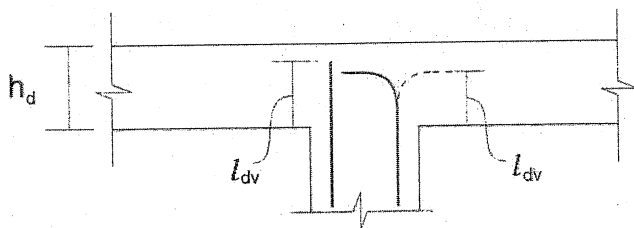
FIGURE 31F-7-9—DEVELOPMENT LENGTH
