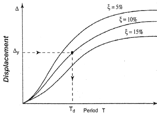
FIGURE 31F-4-4—DESIGN DISPLACEMENT RESPONSE SPECTRA
