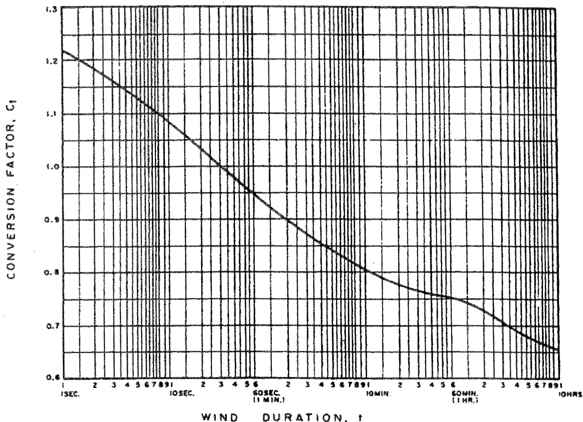
FIGURE 31F-3-3—WINDSPEED CONVERSION FACTOR [3.10]
