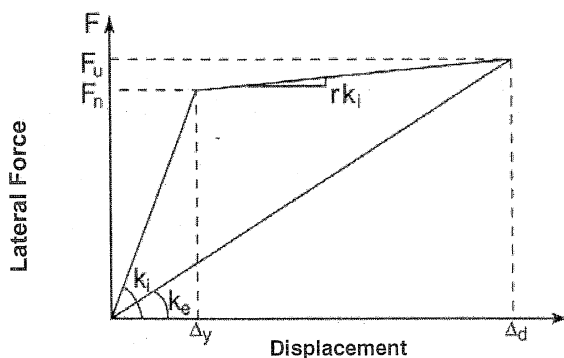
FIGURE 31F-4-5—EFFECTIVE STIFFNESS, k_e [4.1]
