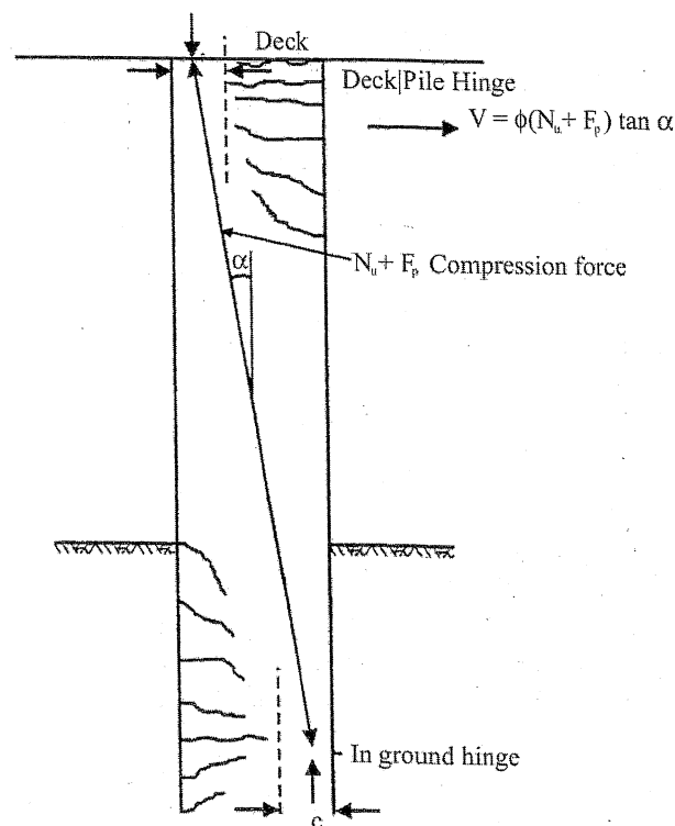
FIGURE 31F-7-8—AXIAL FORCE SHEAR MECHANISM
